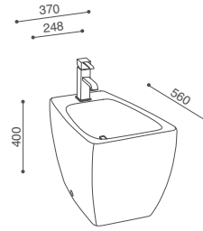
bidet a terra a filo parete floor-standing back-to-wall bidet
