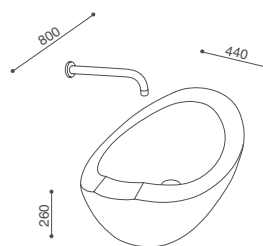
lavabo 80 cm 80 cm basin
