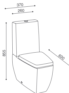
vaso a terra monoblocco con cassetta close coupled floor-standing wc pan with cistem
