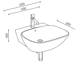
lavabo 55 cm sospeso 55 cm wall-mounted basin
