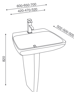
lavabo 60-65-70 cm con colonna 60-65-70 basin with pedestal
