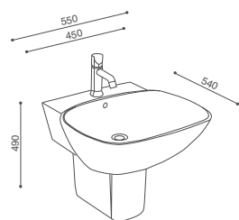
lavabo 55 cm con semi colonna 55 cm basin with semi-pedestal
