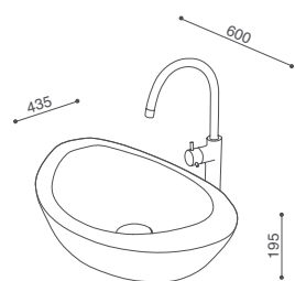
lavabo 60 cm 60 cm basin
