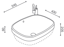
vanity vanity basin
