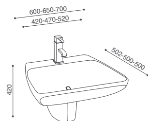
lavabo 60-65-70 cm con semi colonna 60-65-70 basin with semi-pedestal
