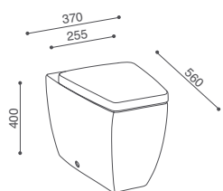
vaso a terra a filo parete floor-standing back-to-wall wc pan
