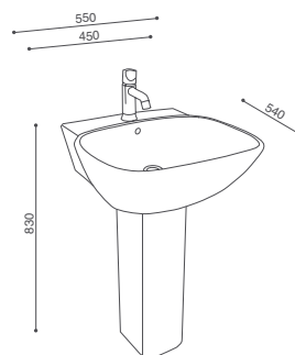
lavabo 55 cm con colonna 55 cm basin with pedestal
