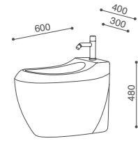
bidet a terra a filo parete floor-standing back-to-wall bidet
