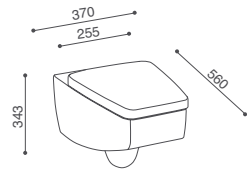
vaso sospeso wall-mounted wc pan
