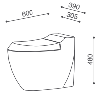
vaso a terra a filo parete floor-standing back-to-wall wc pan
